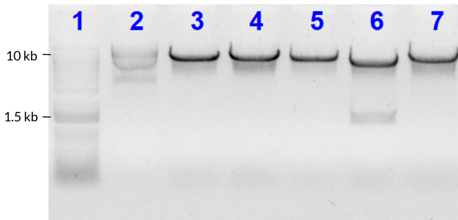
Figure 3. Restriction digest of the final library.
